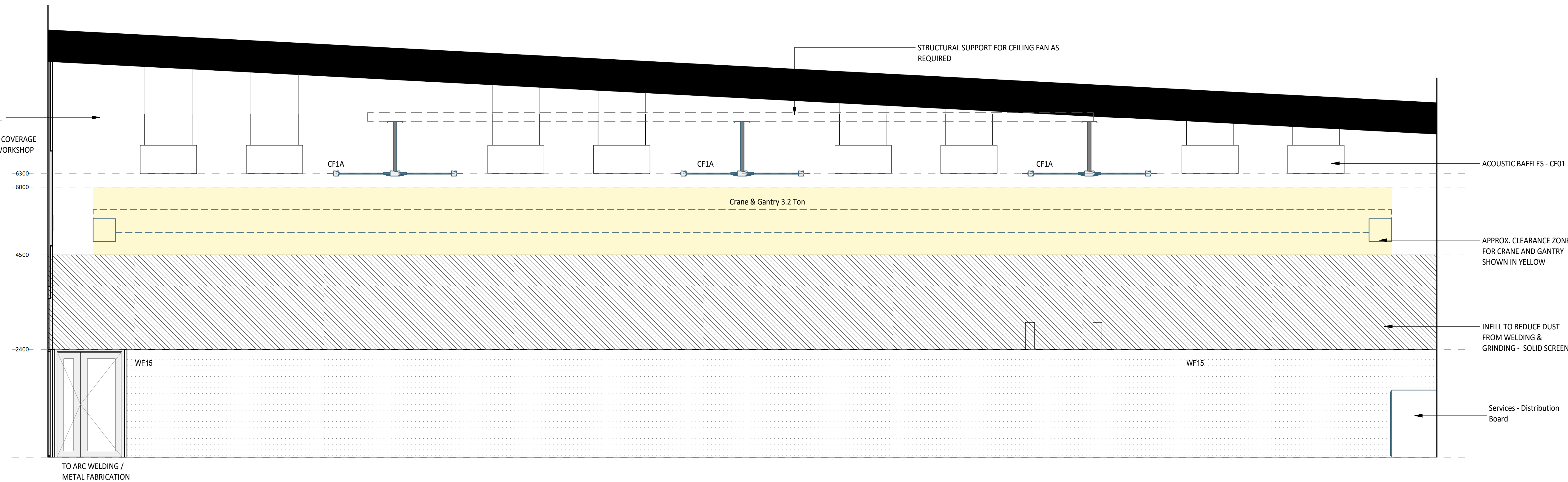
2 ELEVATION DETAIL 60-011 1 : 50
